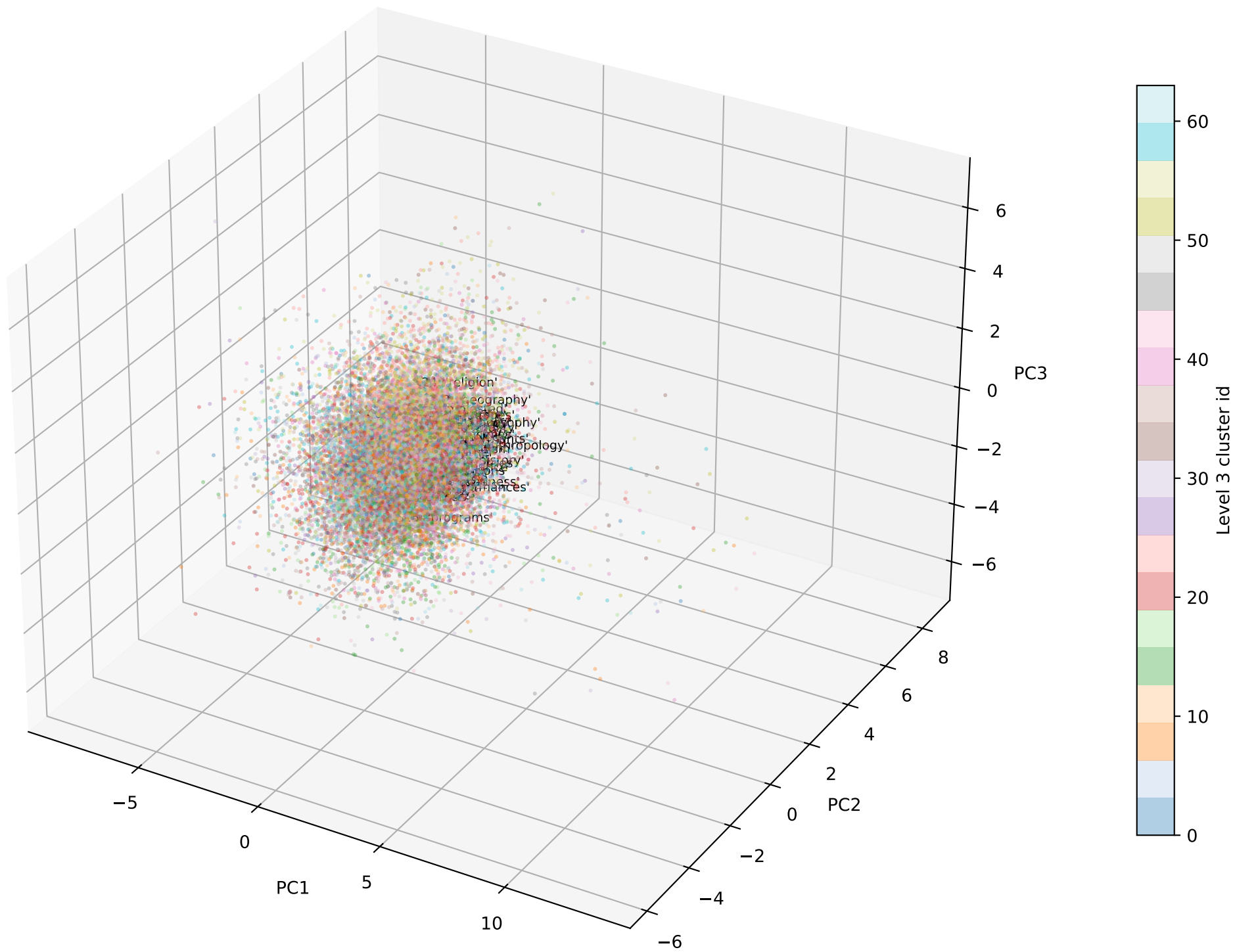
✗ Level 3 centroids
