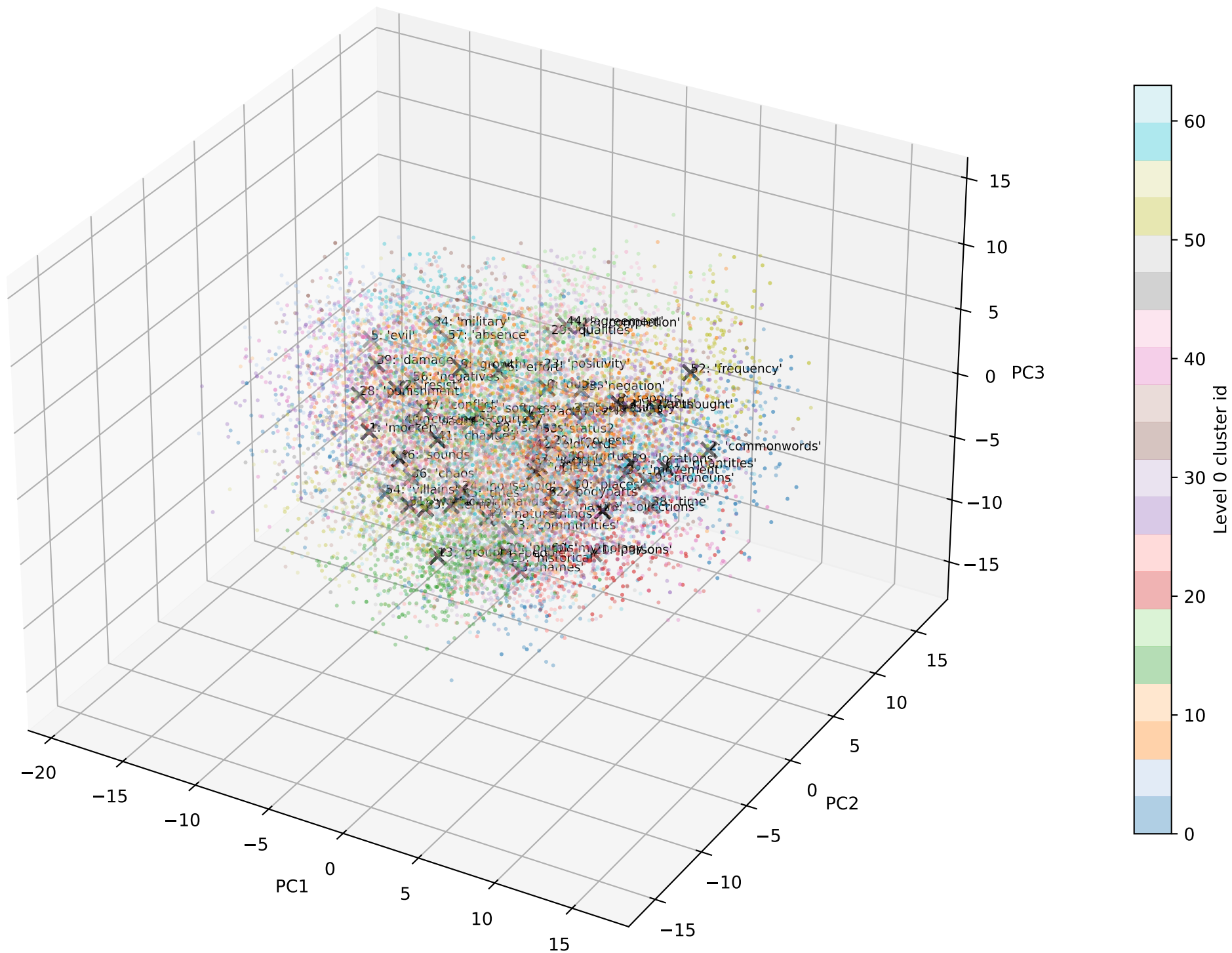
✗ Level 0 centroids
