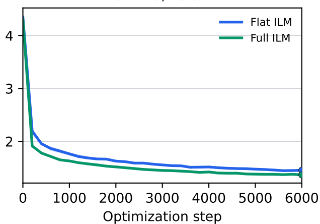
enwik8, 15.5M
