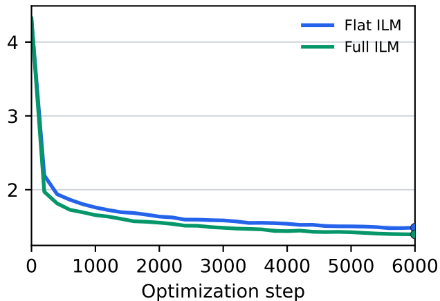
enwik8, 15.5M
