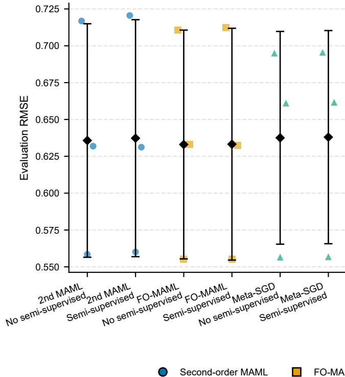
Multi-seed performance on Yellow River data
