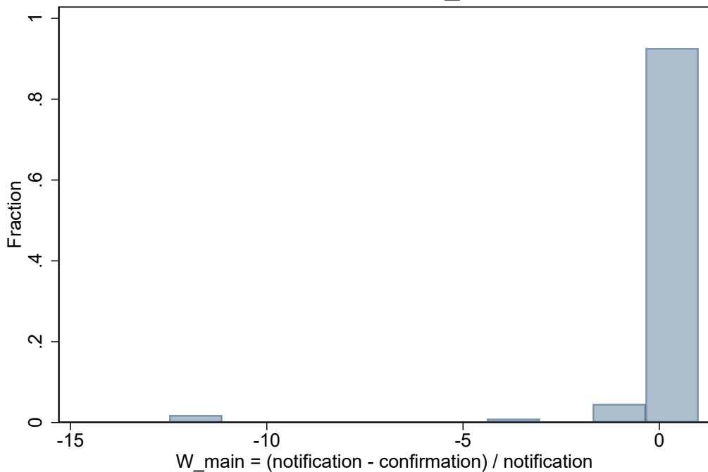
Distribution of W_{\text{main}}
