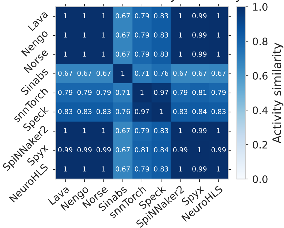
SCNN first-IF activity similarity
