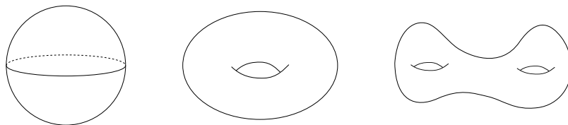
Figure 8.1: Orientable surfaces
