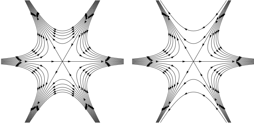
Figure 11.5: Figure 5(Left – F ; Right – \tilde{F} )
