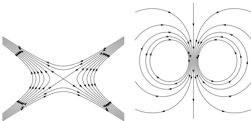
Figure 11.4: Figure 4(Left \iota = -1 ; Right \iota = +2 )
