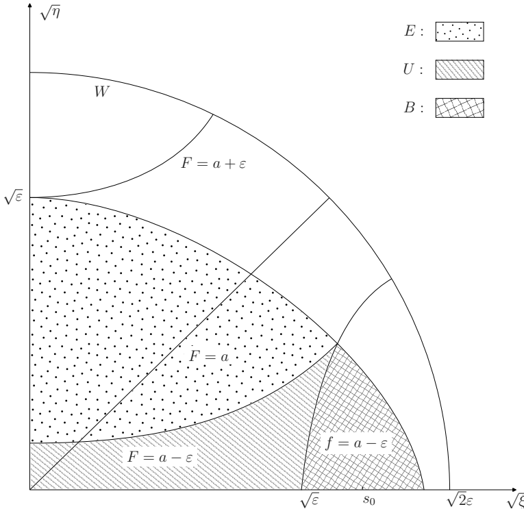
Figure C.2: U hatched; f^{-1}((-\infty, a - \epsilon)) \cap U double-hatched
