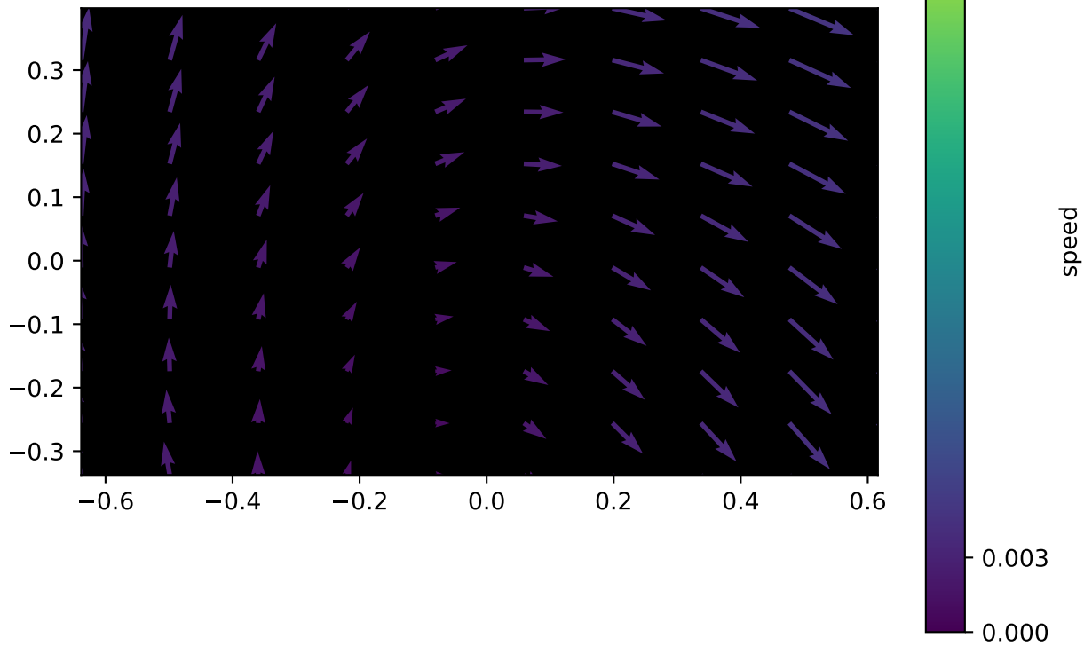
vector field 7 of 10
