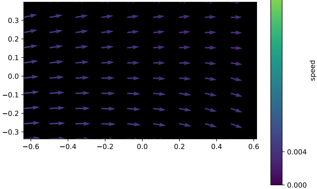
vector field 3 of 10
