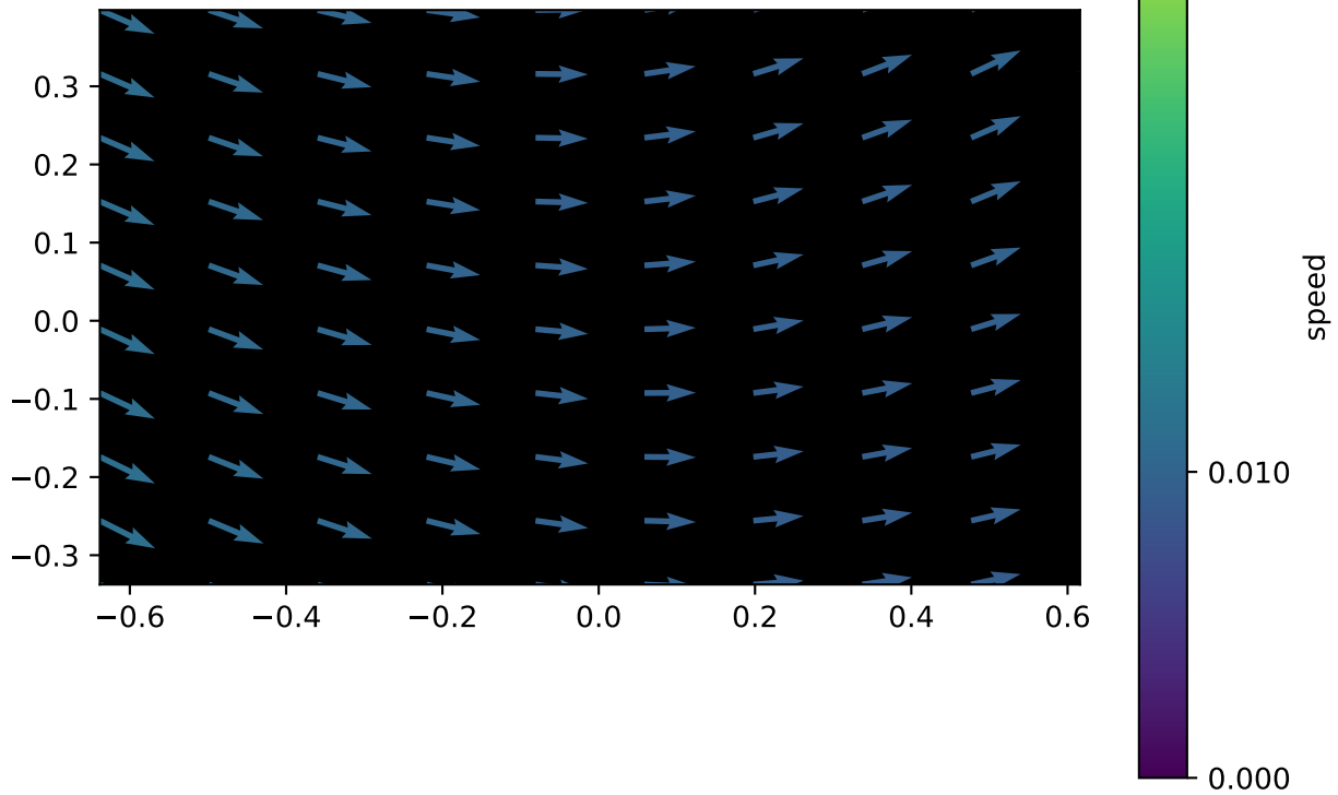
vector field 10 of 10
