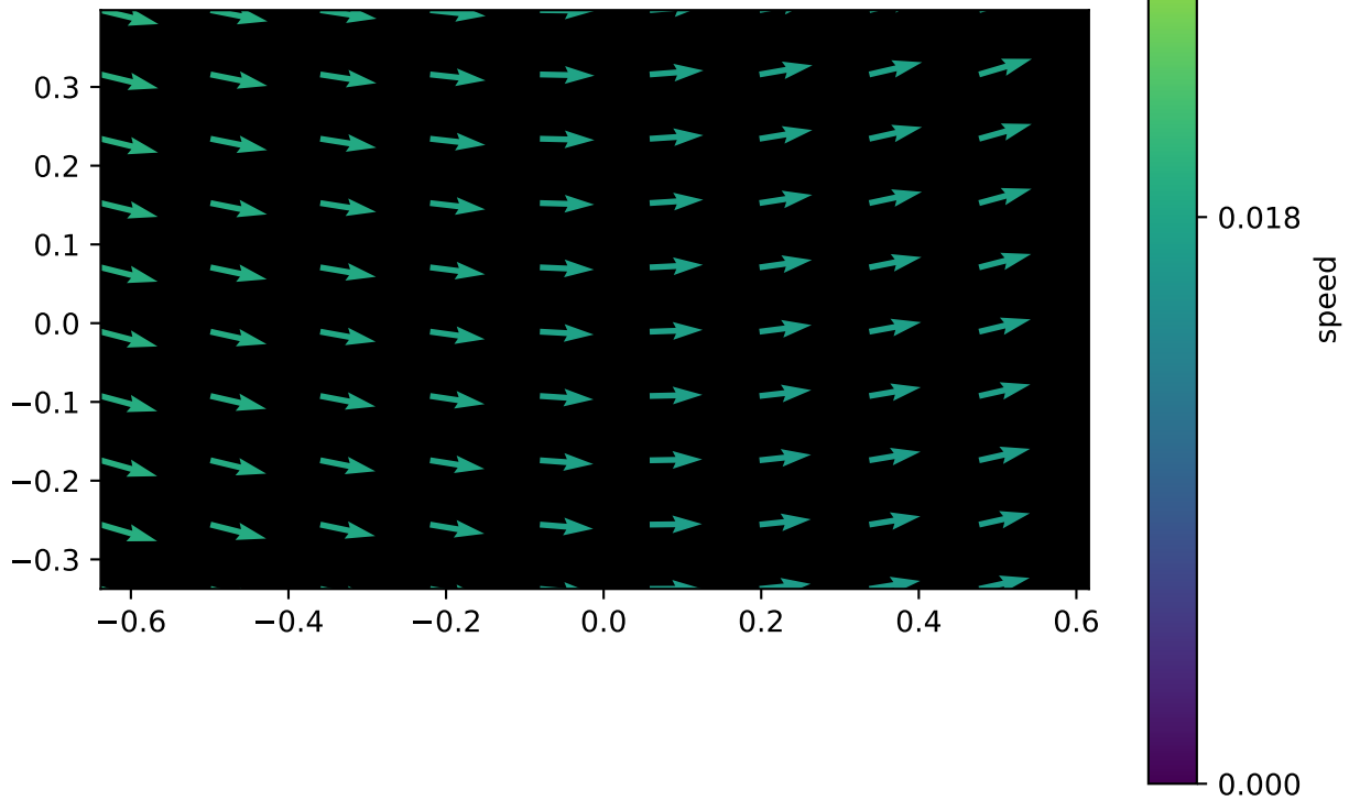
vector field 8 of 10
