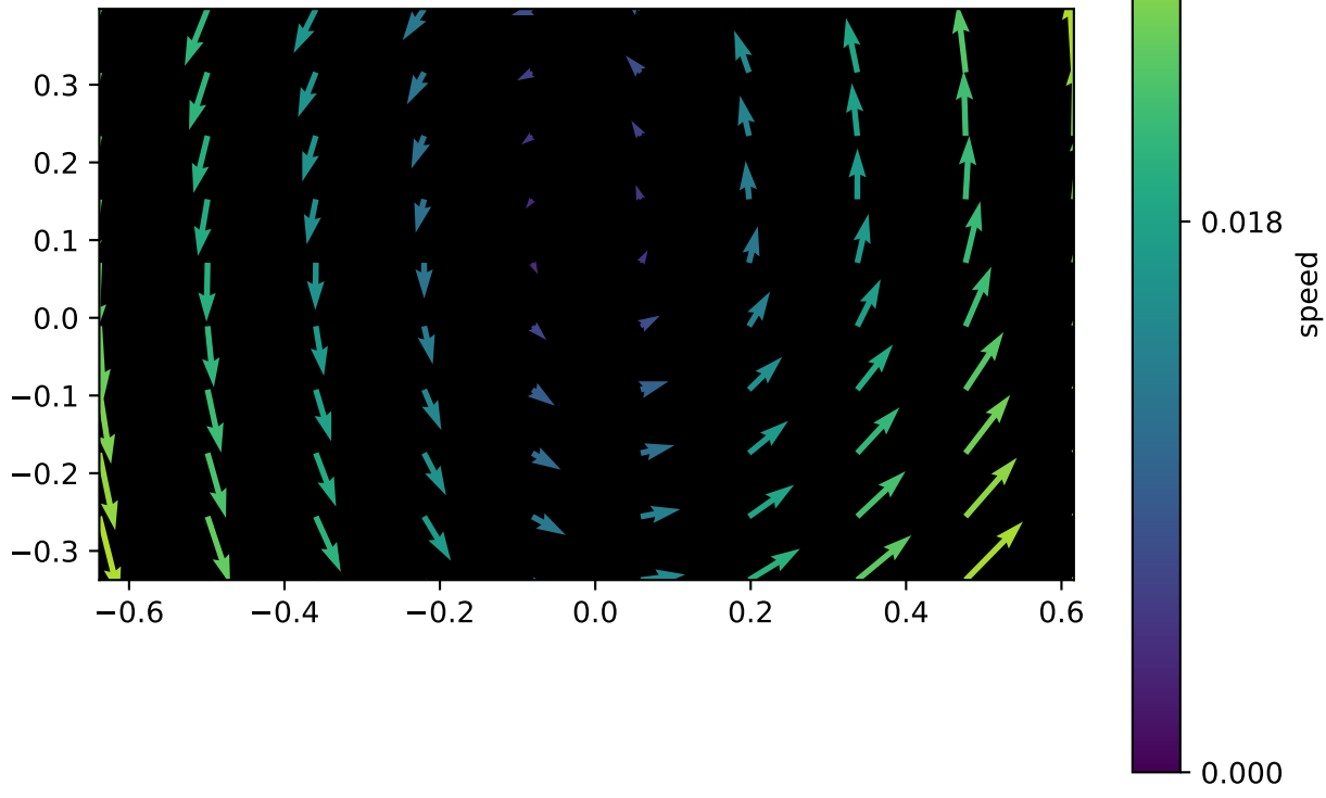
vector field 5 of 10
