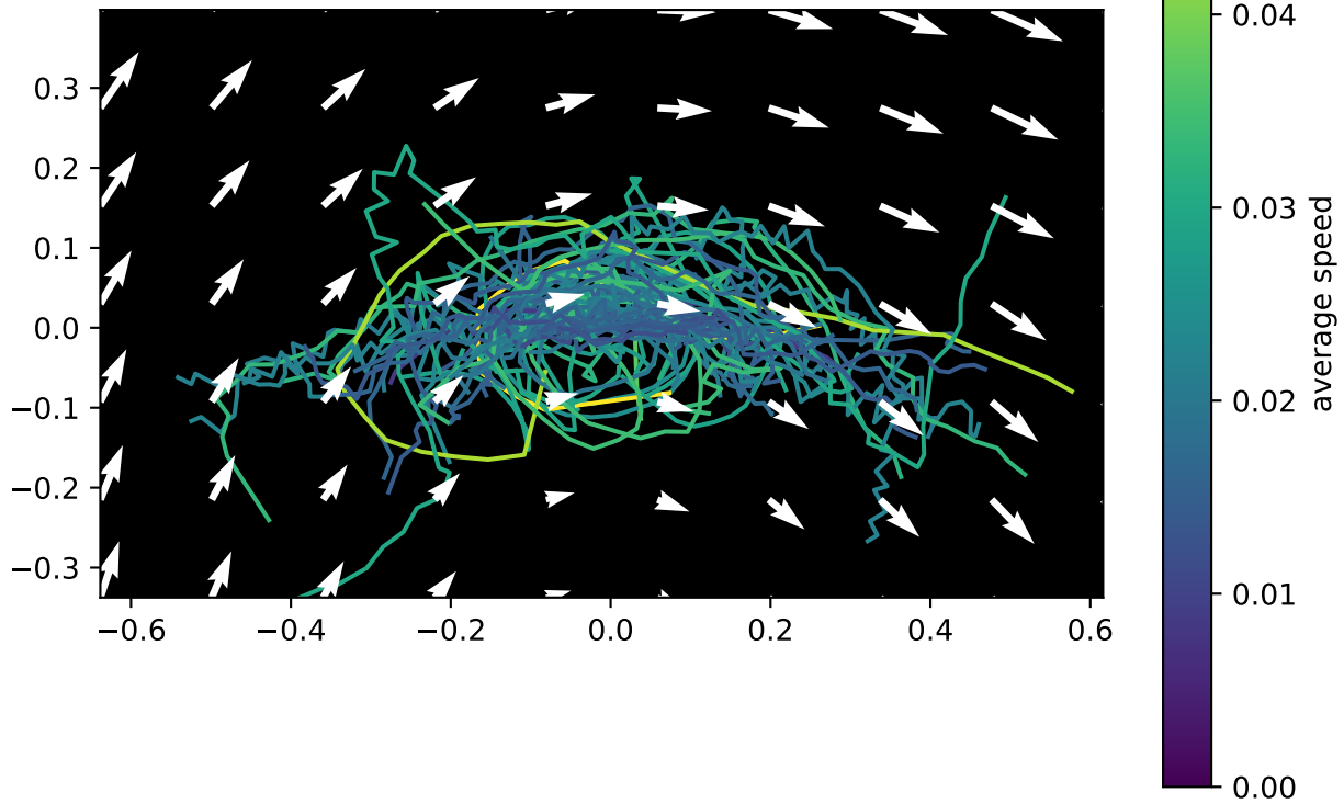
cluster 2 of 6
