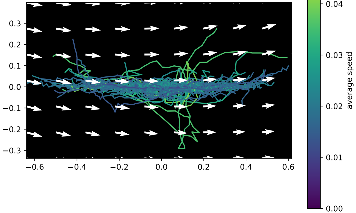
cluster 5 of 6
