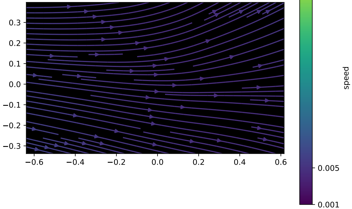
streamplot 3 of 6
