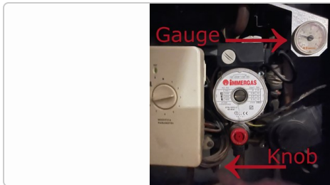
Boiler pressure gauge (keep between 1–2 bar) and fill knob
