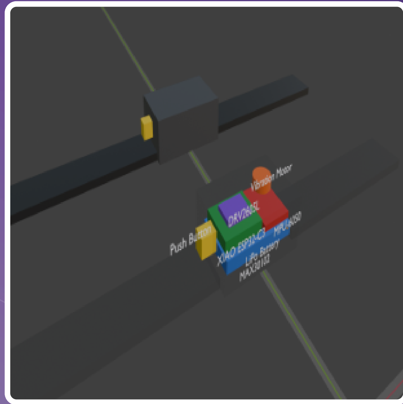
Himbing Smart Watch
