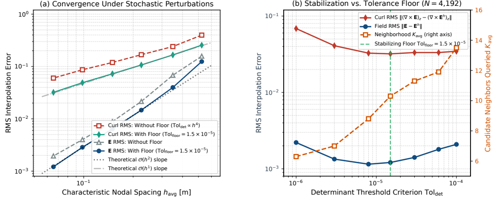
Figure 6: Numerical robustness and conditioning analysis for the 2D VNMM complete base \mathcal{P}^1 under stochastic perturbations (uniform nodal jitter of 25% and random director angles \theta_i \in [0, 2\pi) ) over \Omega = [0, \pi]^2 : (a) Convergence under stochastic mesh refinement with and without the determinant tolerance floor, highlighting curl degradation when scaling \text{Tol}_{\text{det}} \propto h^4 without a floor due to ill-conditioned sextets ( \kappa(\mathbf{A}) > 180 ) and restored strict monotonic convergence when applying \text{Tol}_{\text{floor}} = 1.5 \times 10^{-5} ; (b) Interpolation error and candidate search neighborhood K_{\text{avg}} as a function of the threshold criterion \text{Tol}_{\text{det}} for the fine grid ( N = 4,192 ), identifying the stable operating regime for \text{Tol}_{\text{det}} \geq 1.5 \times 10^{-5} .
