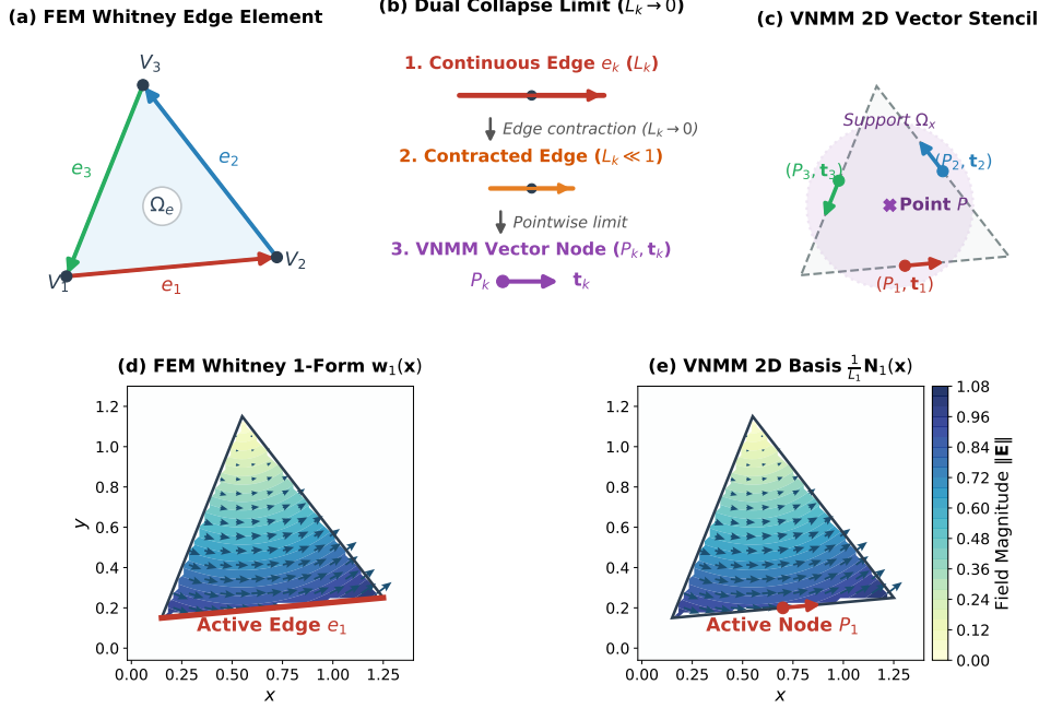
Figure 1: Exact topological and algebraic dual equivalence between lowest-order Whitney edge elements (FEM 1-forms) and the VNMM 2D \mathcal{L}^1 meshless vector formulation: (a) Primal triangular cell \Omega_e with vertices V_1, V_2, V_3 and oriented edges e_1, e_2, e_3 ; (b) Conceptual dual collapse limit as edge length contracts ( L_k \rightarrow 0 ), identifying the discrete circulation integral L_k^{-1} \int_{e_k} \vec{E} \cdot \vec{t}_k ds directly with the tangential projection at a point, e_k = \vec{E}(P_k) \cdot \vec{t}_k ; (c) VNMM 2D meshless support stencil with vector nodes (P_k, \vec{t}_k) placed at the edge midpoints and compact support \Omega_x ; (d) Vector field and magnitude contour of the Whitney 1-form \vec{w}_1(\mathbf{x}) = \lambda_1 \nabla \lambda_2 - \lambda_2 \nabla \lambda_1 associated with active edge e_1 ; (e) Vector field and magnitude contour of the normalized VNMM \mathcal{L}^1 vector basis function \frac{1}{L_1} \vec{N}_1(\mathbf{x}) associated with active node (P_1, \vec{t}_1) . Both fields are algebraically identical over \Omega_e , satisfying \|\vec{w}_1(\mathbf{x}) - L_1^{-1} \vec{N}_1(\mathbf{x})\|_{L^\infty(\Omega_e)} \leq 2.2 \times 10^{-16} .
