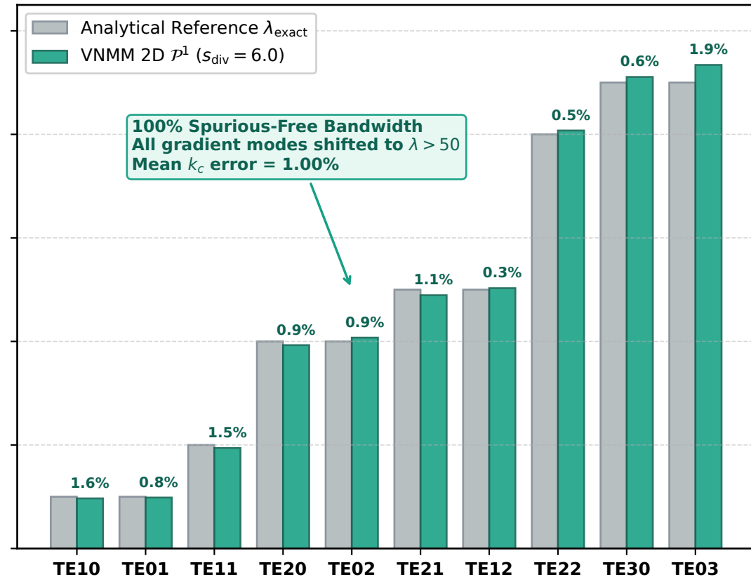
(b) Div-Curl Regularized Formulation ( s_{\text{div}} = 6.0 ) Total Spectral Purification of Useful Bandwidth
