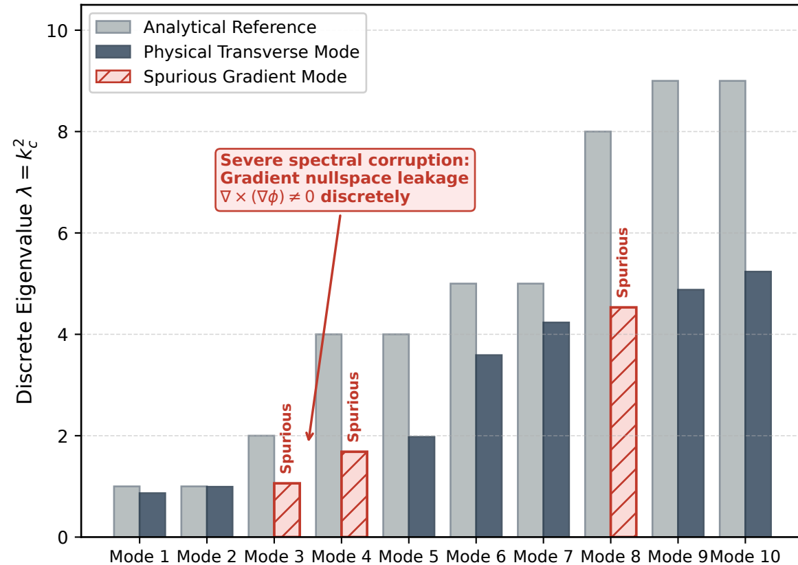
(a) Unregularized Formulation ( s_{\text{div}} = 0.0 ) Proliferation of Spurious Gradient Modes ( \mathbf{E} = \nabla\phi )
