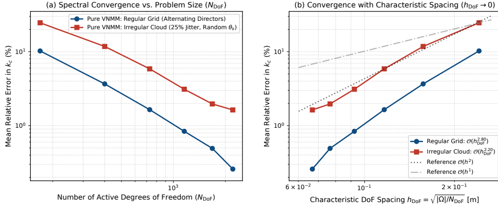
Figure 9: Comparative spectral convergence study across 6 refinement levels ( N \in \{9, 13, 17, 21, 25, 29\} ) under spatial and directional disorder: (a) Mean relative spectral error in cutoff wavenumber k_c (%) as a function of total active degrees of freedom N_{\text{DoF}} ; (b) Convergence rate as a function of characteristic DoF spacing h_{\text{DoF}} = \sqrt{|\Omega|/N_{\text{DoF}}} . The regular grid exhibits an observed fitted slope of \mathcal{O}(h_{\text{DoF}}^{2.80}) , while the irregular cloud (25% spatial jitter and random director orientations \theta_k \in [0, 2\pi) ) exhibits an observed fitted slope of \mathcal{O}(h_{\text{DoF}}^{2.20}) across the evaluated single-realization sequence, which is empirically compatible with the expected behavior of a complete linear polynomial approximation.
