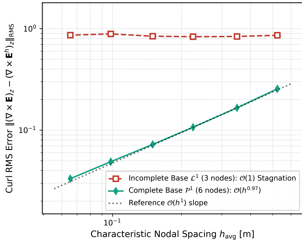
(b) Curl Operator Convergence ( (\nabla \times \mathbf{E})_z )
