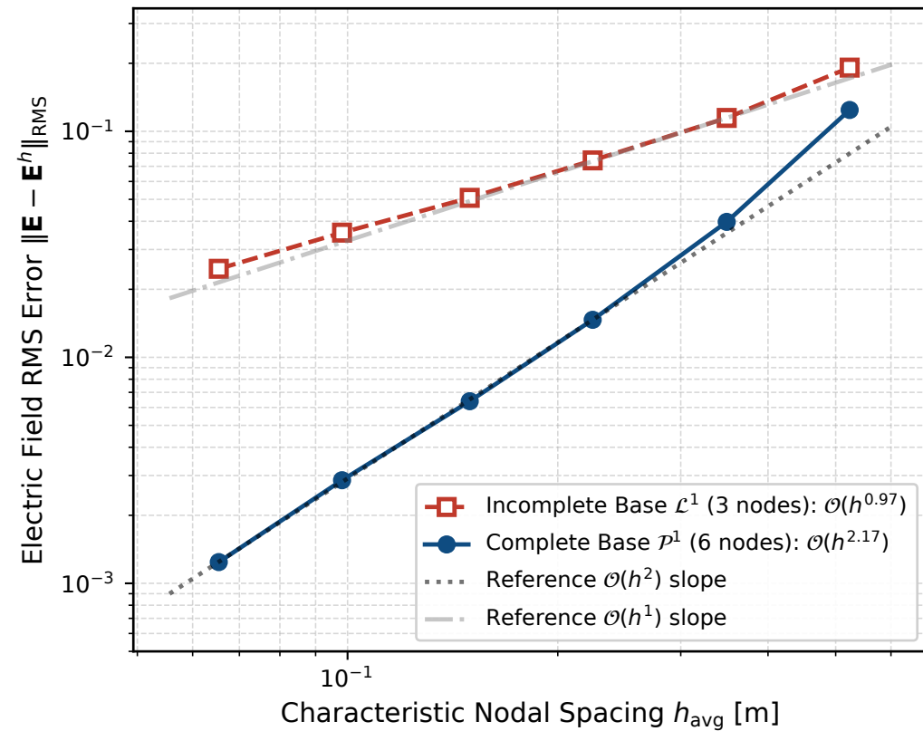
(a) Electric Field Convergence ( \mathbf{E} )
