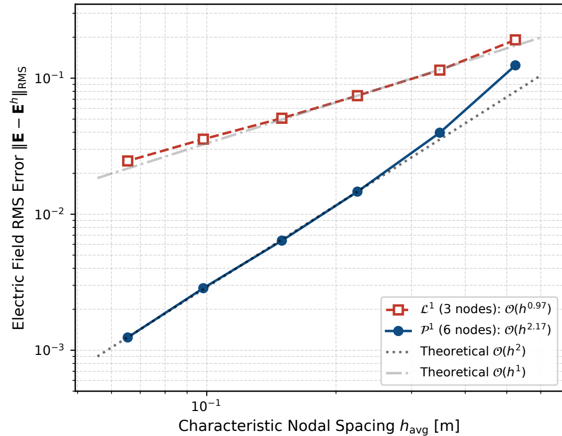
(a) Electric Field Convergence ( \mathbf{E} )
