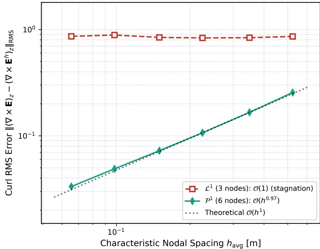
(b) Curl Operator Convergence ( (\nabla \times \mathbf{E})_z )
