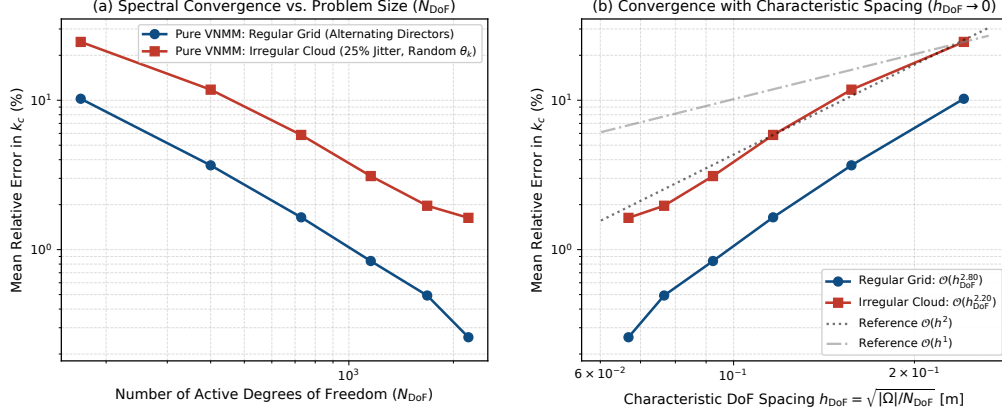
Figure 9: Comparative spectral convergence study across 6 refinement levels ( N \in \{9, 13, 17, 21, 25, 29\} ) under spatial and directional disorder: (a) Mean relative spectral error in cutoff wavenumber k_c (%) as a function of total active degrees of freedom N_{\text{DoF}} ; (b) Convergence rate as a function of characteristic DoF spacing h_{\text{DoF}} = \sqrt{|\Omega|/N_{\text{DoF}}} . The regular grid exhibits an observed fitted slope of \mathcal{O}(h_{\text{DoF}}^{2.80}) , while the irregular cloud (25% spatial jitter and random director orientations \theta_k \in [0, 2\pi) ) exhibits an observed fitted slope of \mathcal{O}(h_{\text{DoF}}^{2.20}) \approx \mathcal{O}(h^2) , in close agreement with the theoretical quadratic rate of complete linear polynomials.
