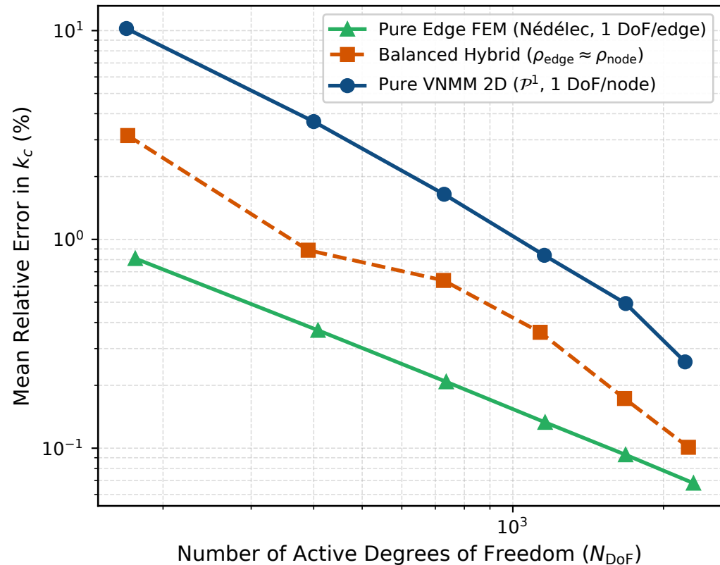
(a) Spectral Convergence vs. Problem Size ( N_{\text{DoF}} )
