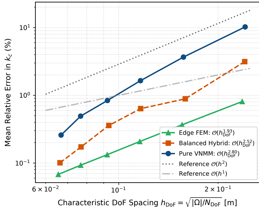
(b) Convergence with Characteristic Spacing ( h_{\text{DoF}} \rightarrow 0 )
