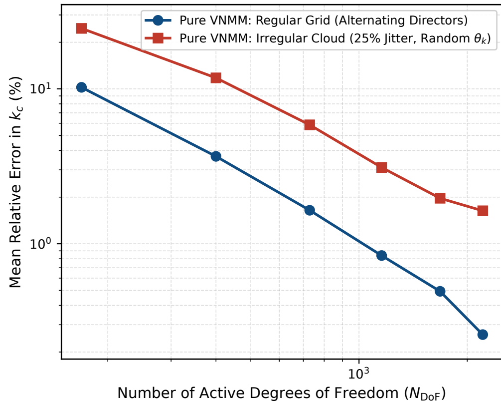
(a) Spectral Convergence vs. Problem Size ( N_{\text{DoF}} )
