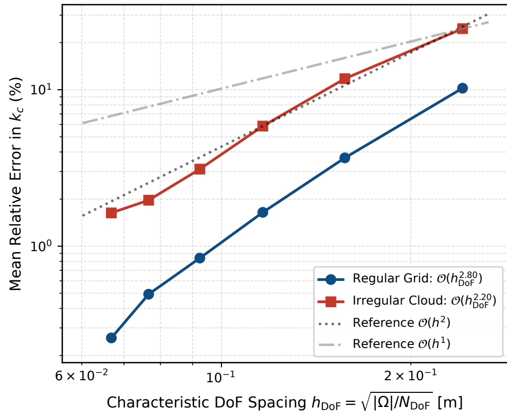
(b) Convergence with Characteristic Spacing ( h_{\text{DoF}} \rightarrow 0 )
