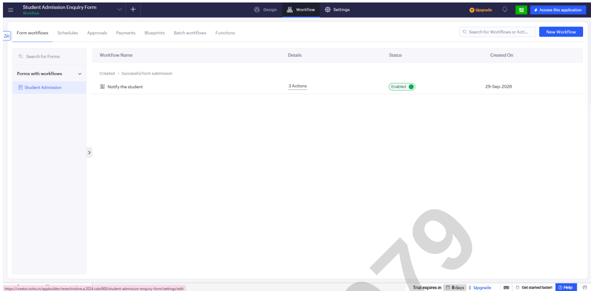
Fig 2.5: Form workflows list showing the Notify the student workflow still enabled
