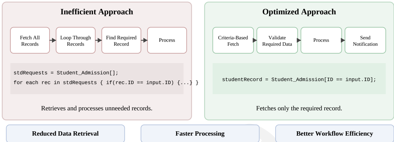
Figure 2: Inefficient and Optimized Approaches (Conceptual Diagram)
