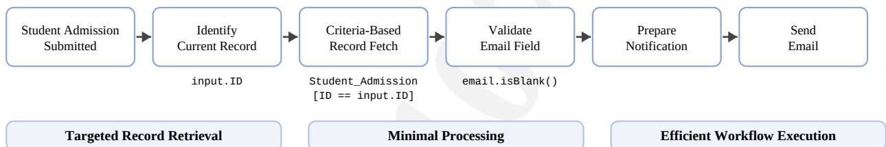
Figure 4: Optimized Student Admission Workflow (Conceptual Diagram)
