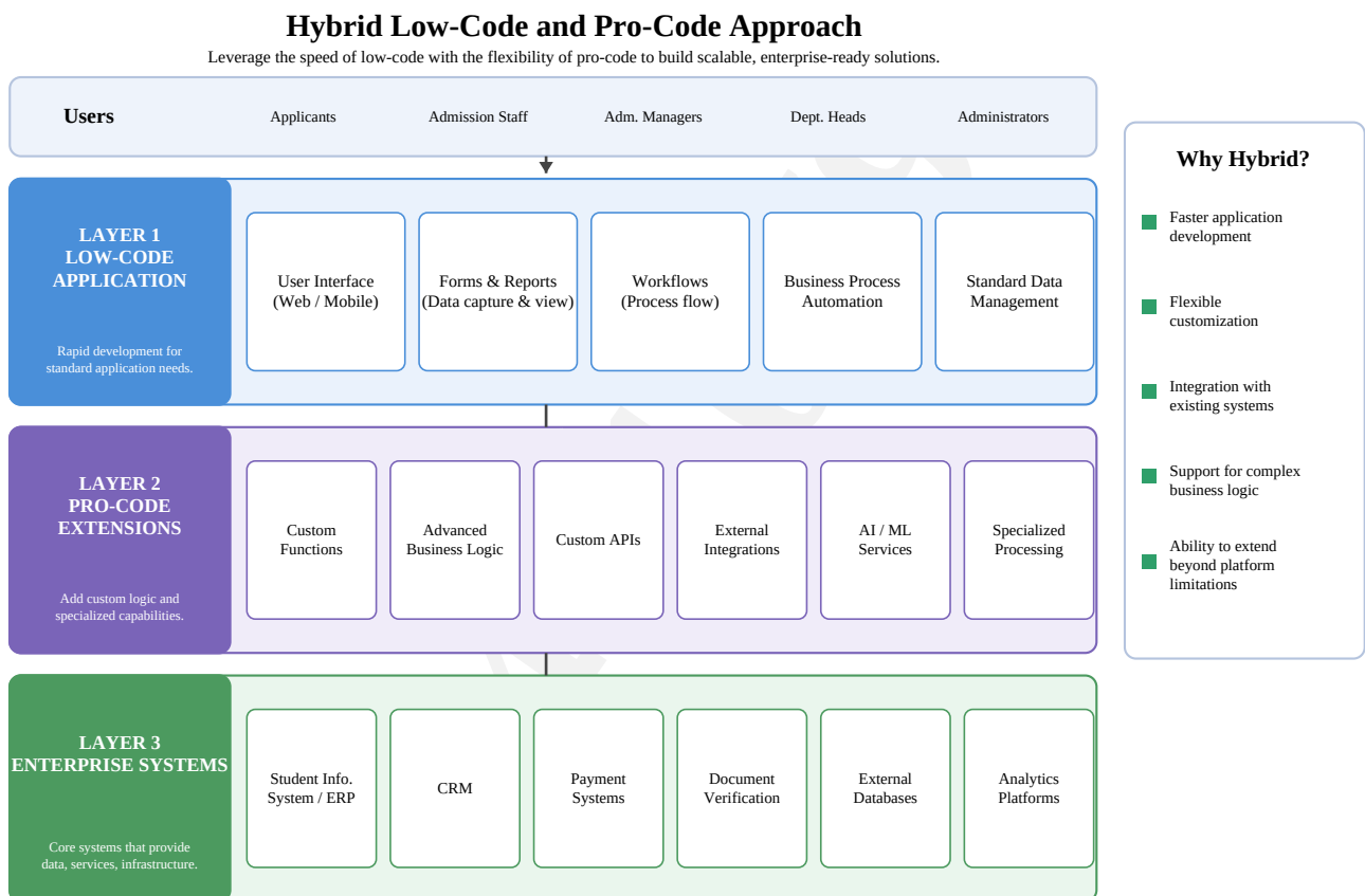
Figure 3: Hybrid Low-Code and Pro-Code Enterprise Architecture
