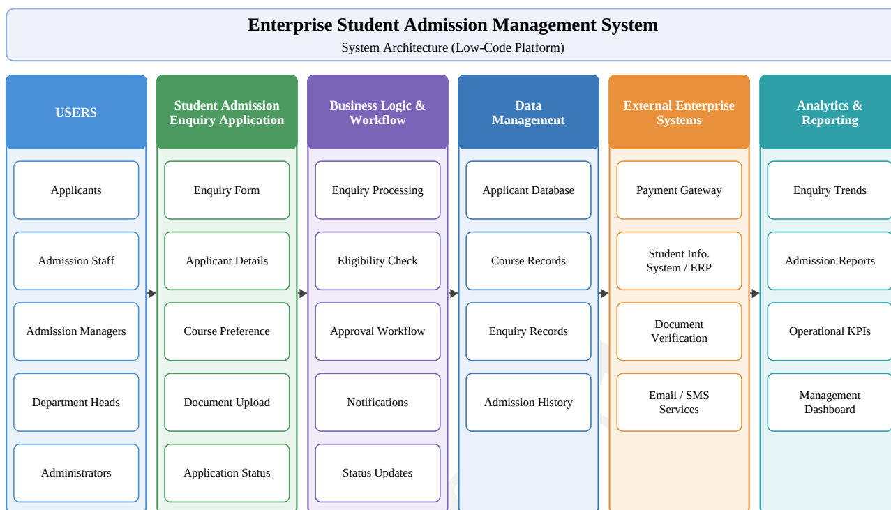
Figure 1: Enterprise Student Admission Management System Architecture
