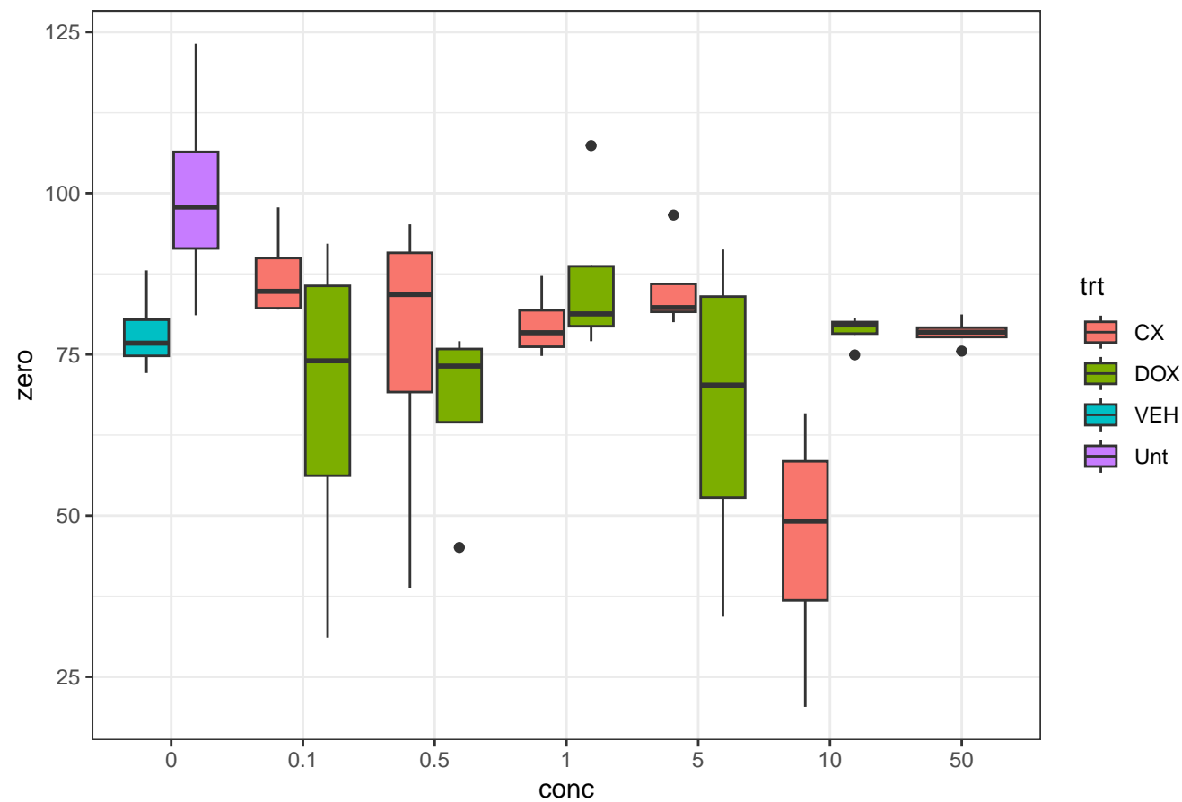
Box plot of normalized day zero across treatments
