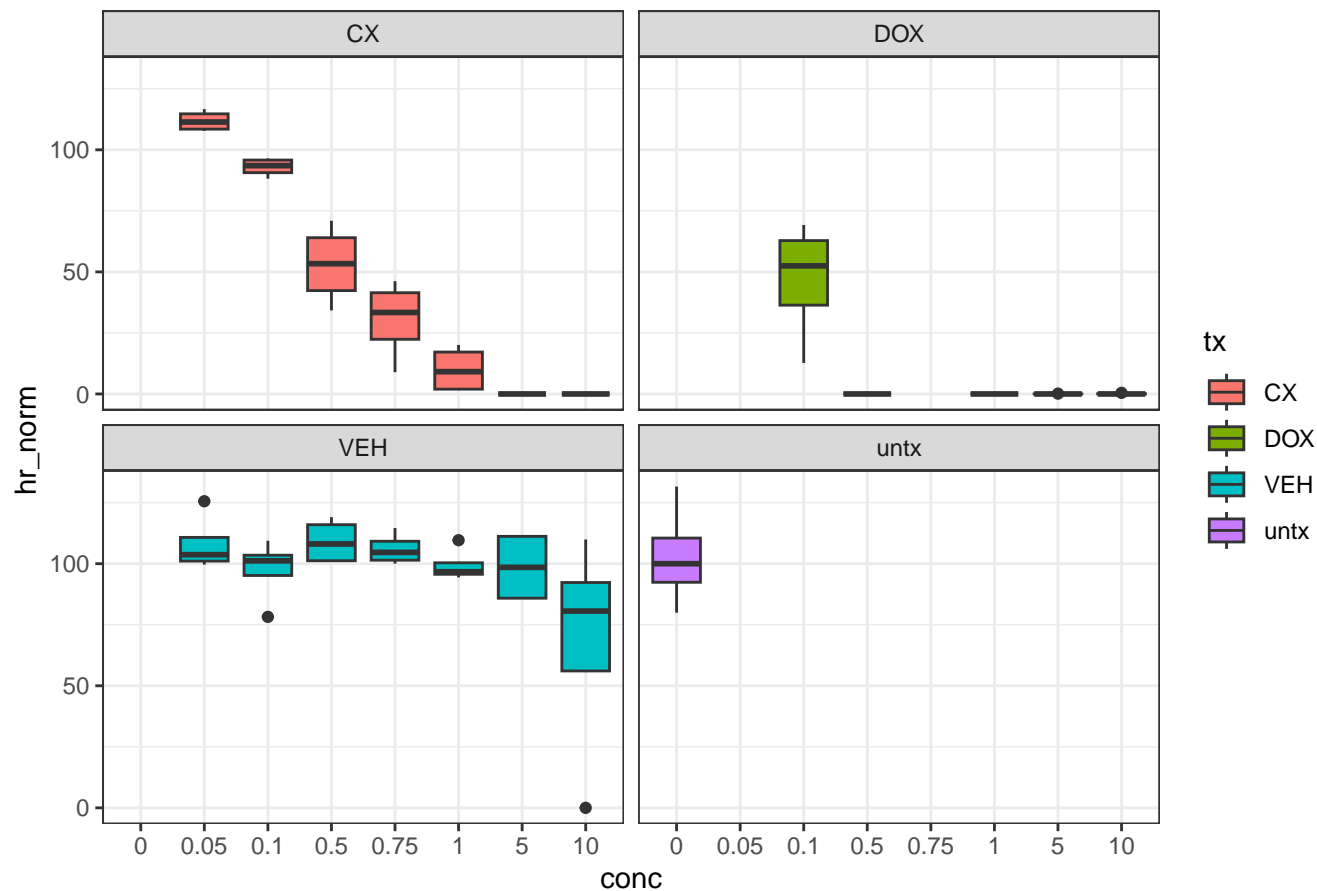
Box plot of normalized 87 DRC
