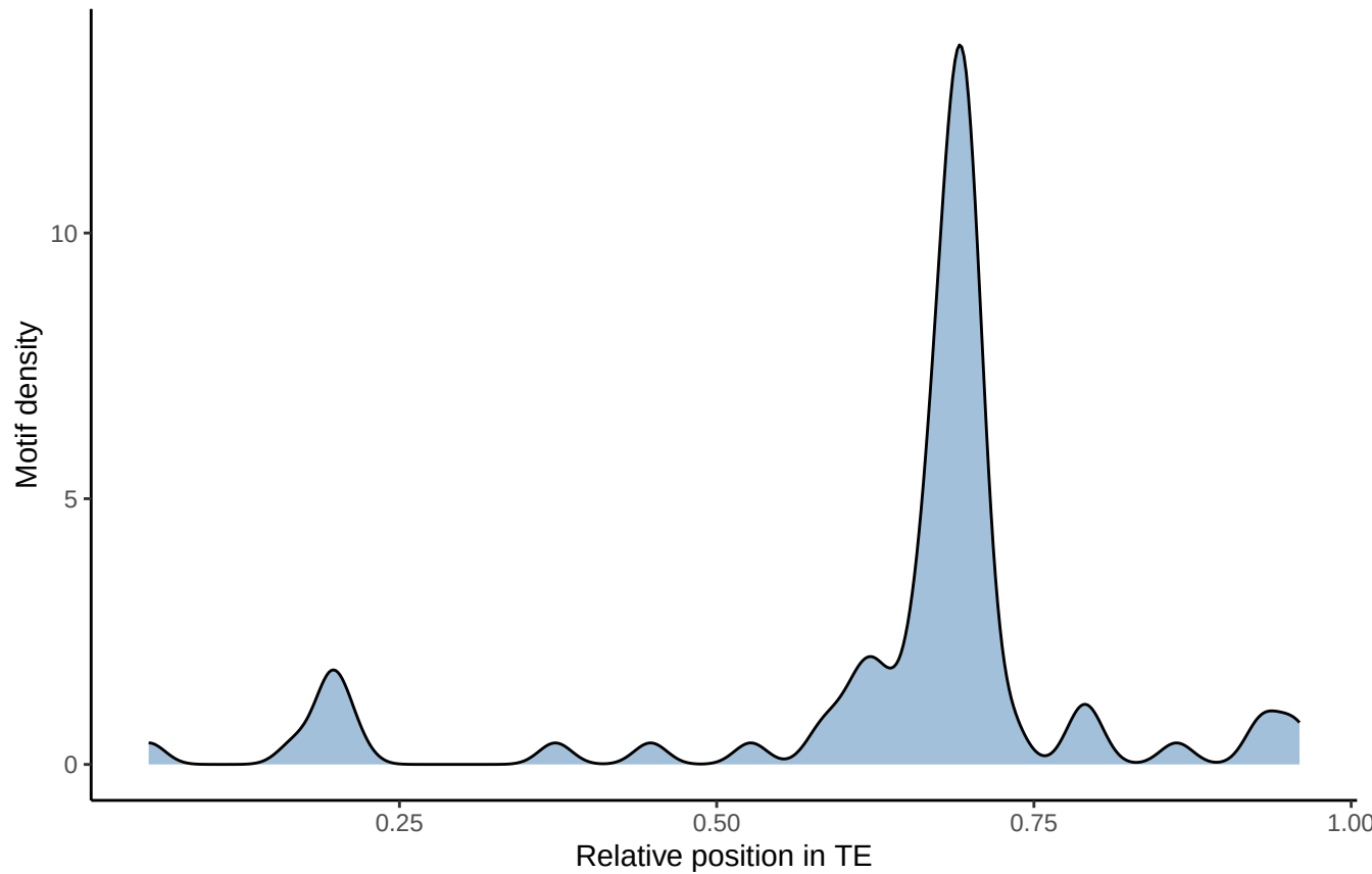
Motif distribution: fimo_out_37 MEME-28
