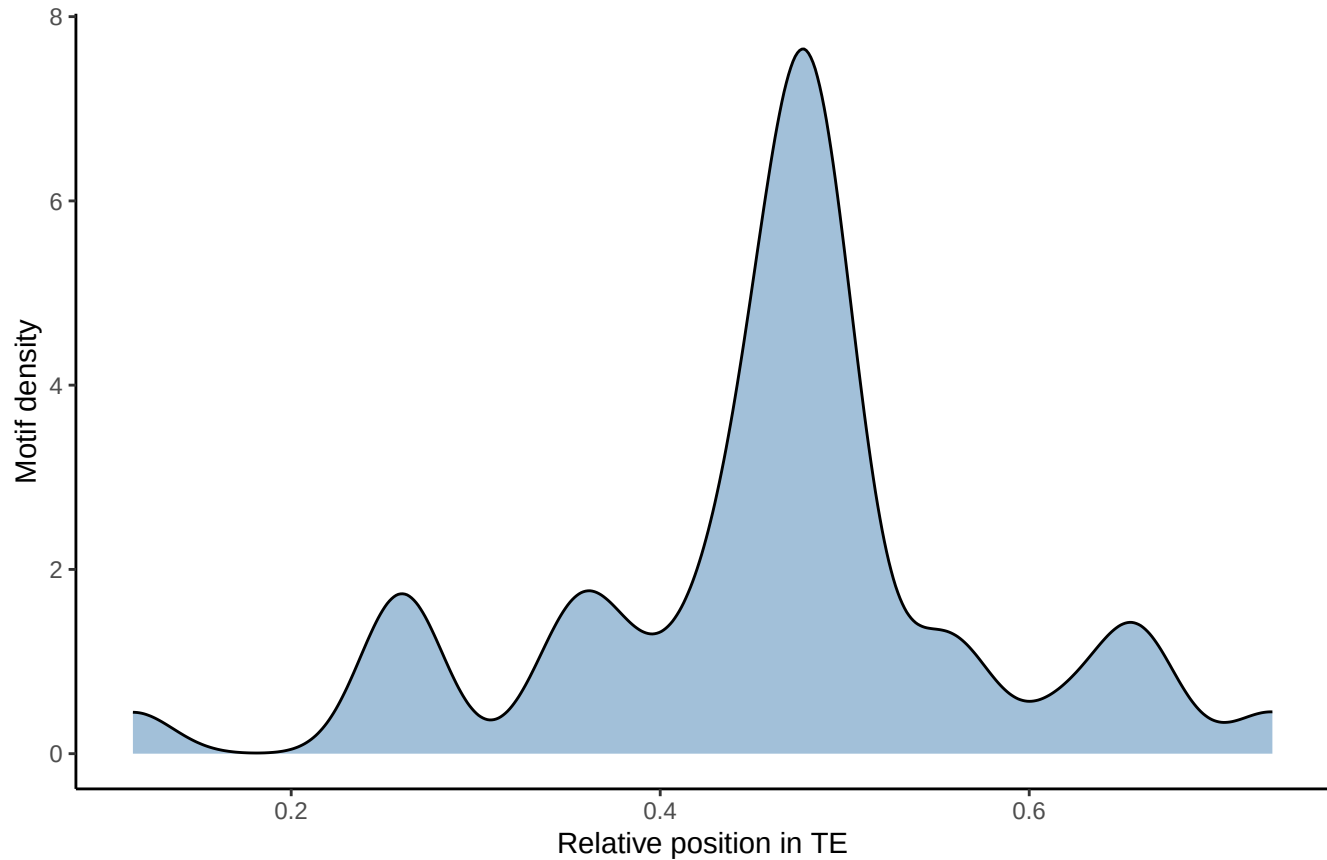
Motif distribution: fimo_out_43 MEME-40
