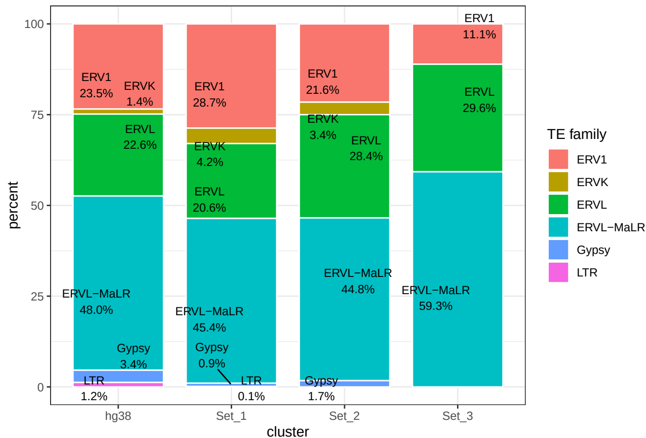
TE Family composition among TE-overlapping ROI summits per set H3K9me3
