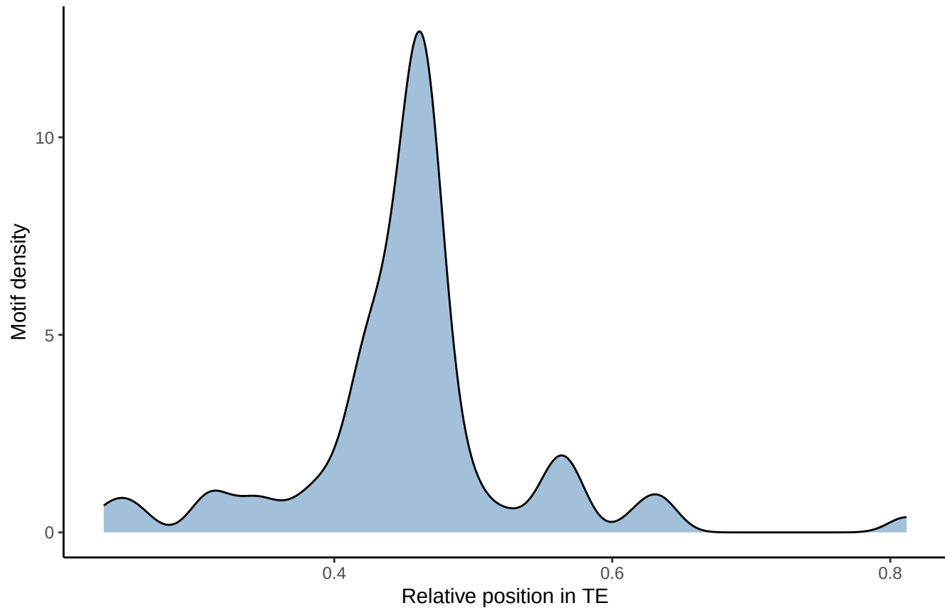
Motif distribution: fimo_out_23 STREME-7
