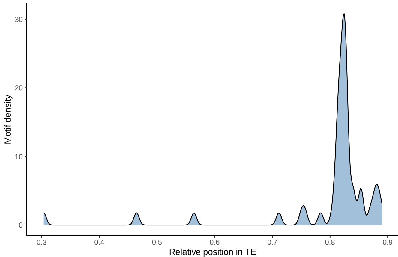
Motif distribution: fimo_out_38 MEME-33
