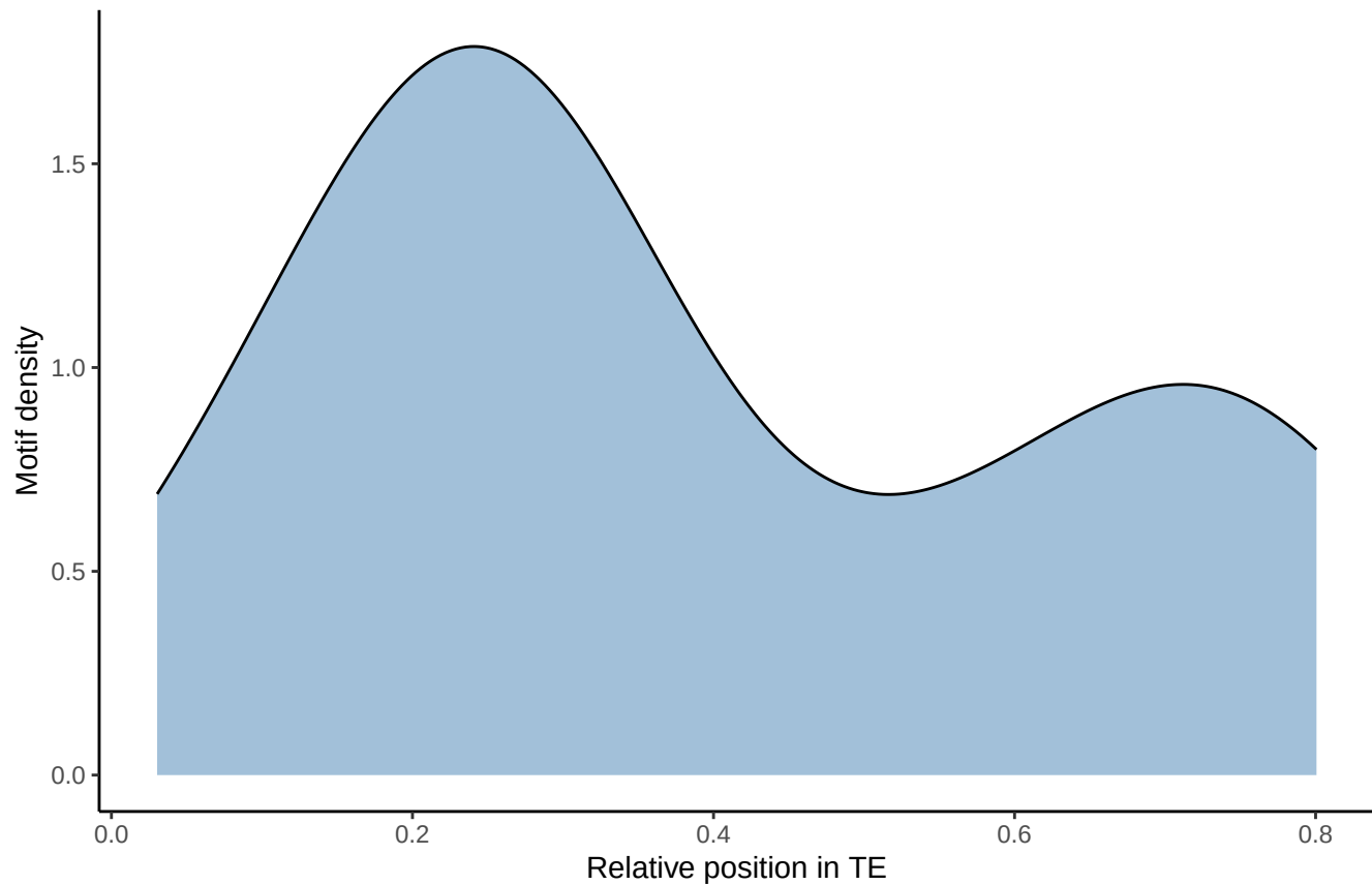
Motif distribution: fimo_out_49 MEME-42
