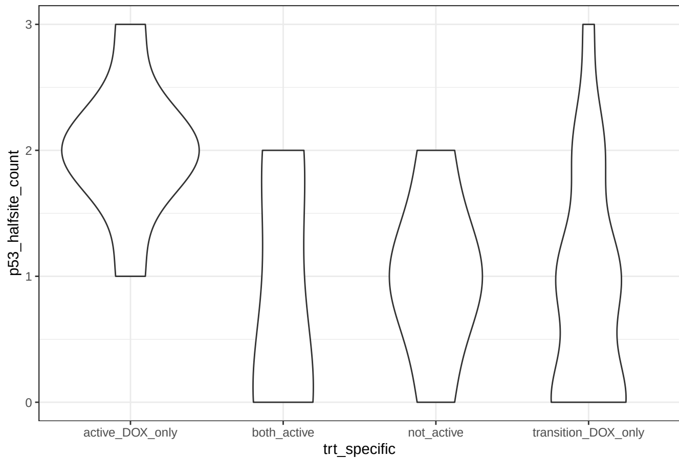
Looking at LTR10E number of halfsites
