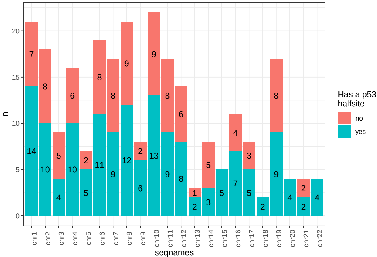
LTR10E distribution across chromosomes with p53halfsite
