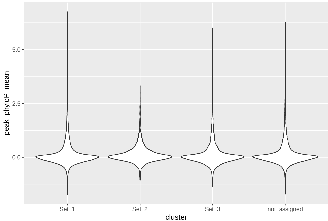
mean phyloP score of all H3K27ac regions
