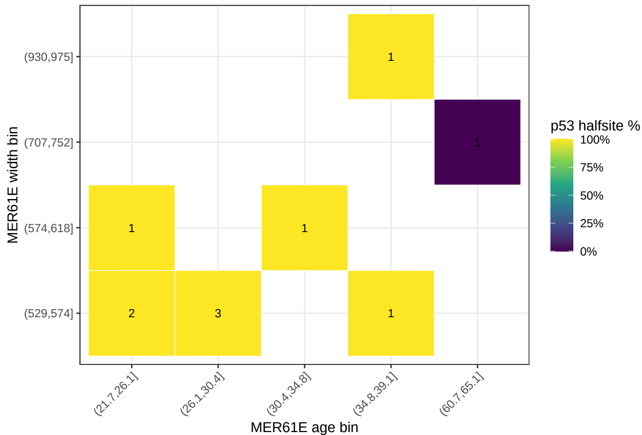
Active_DOX only MER61E p53 breakdown
