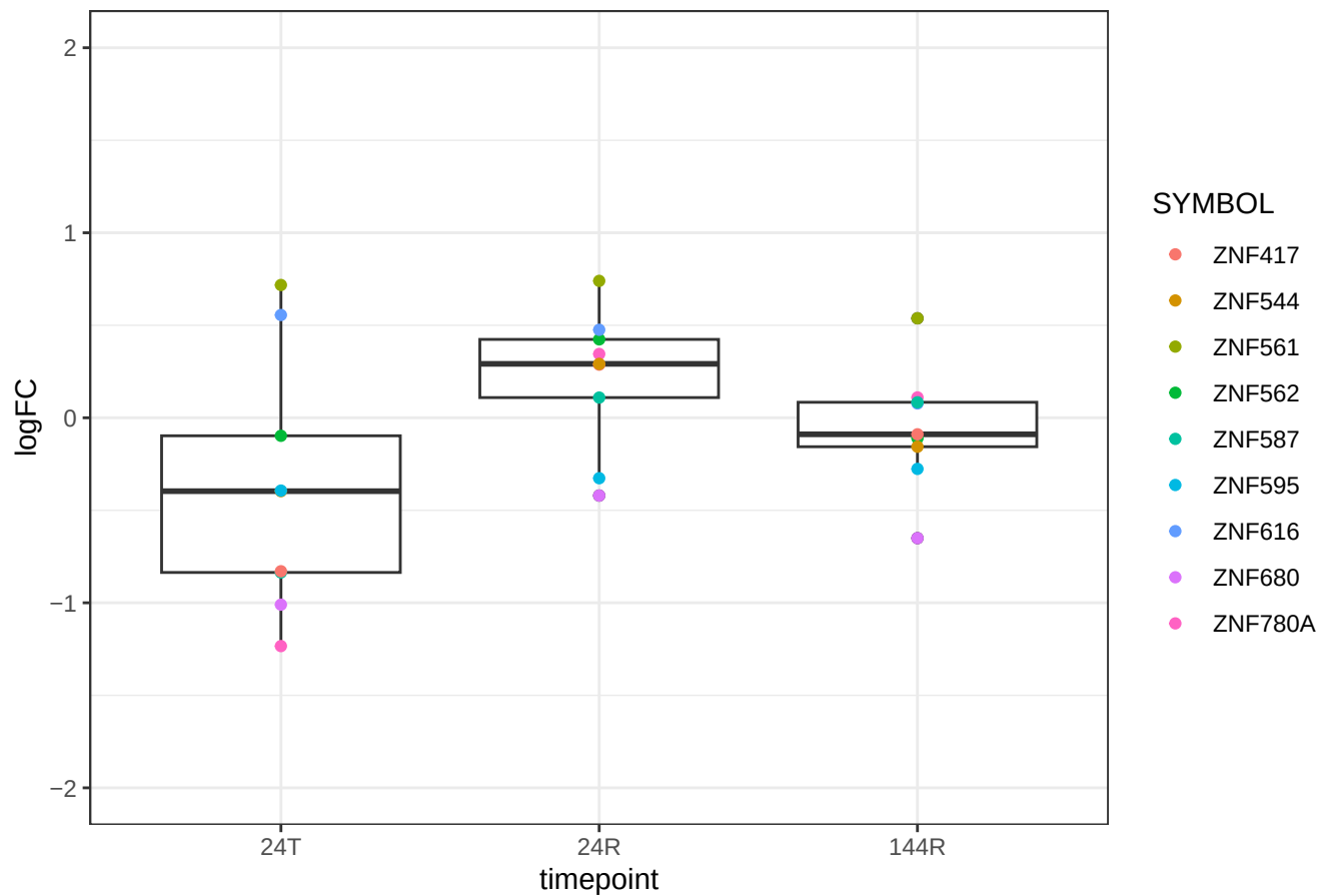
LFC of KZFPs that target specific ERV1 subfamilies
