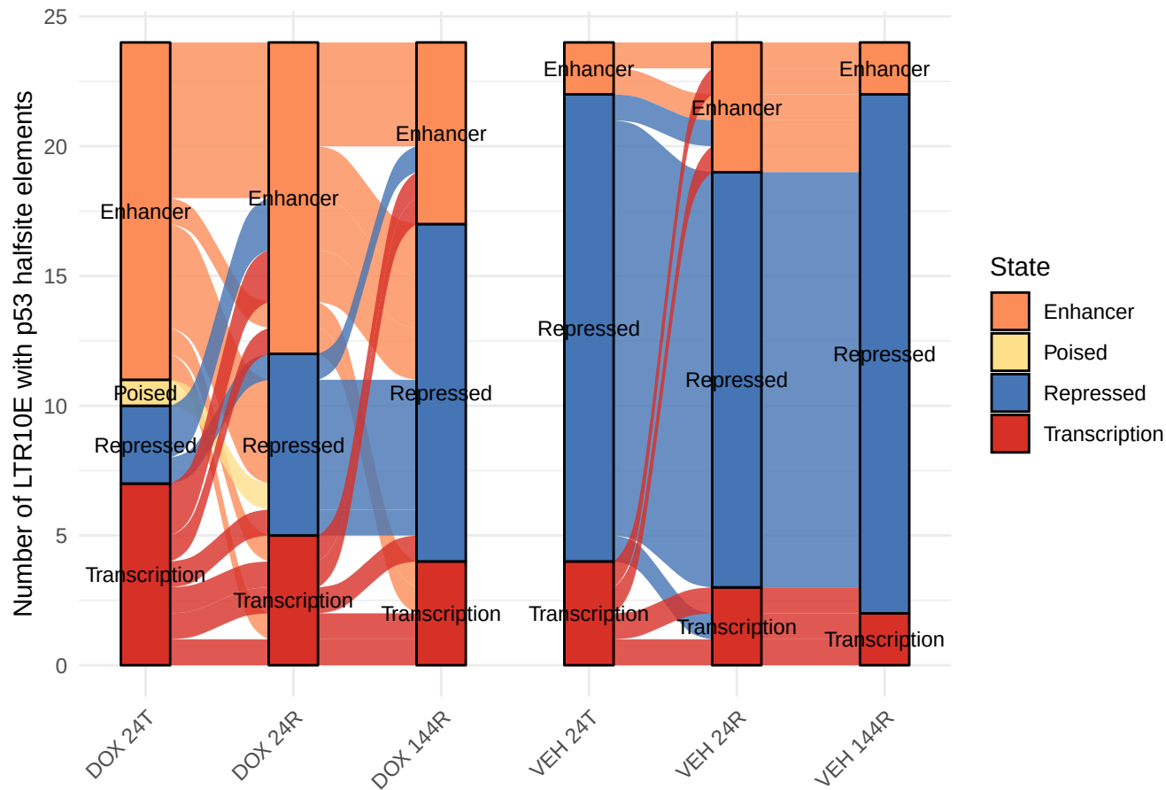
LTR10E with p53 halfsite regulatory-state trajectories
