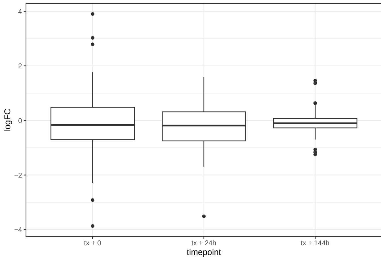
LFC at timepoints of genes nearest to all MER61E TE (chipseeker)
