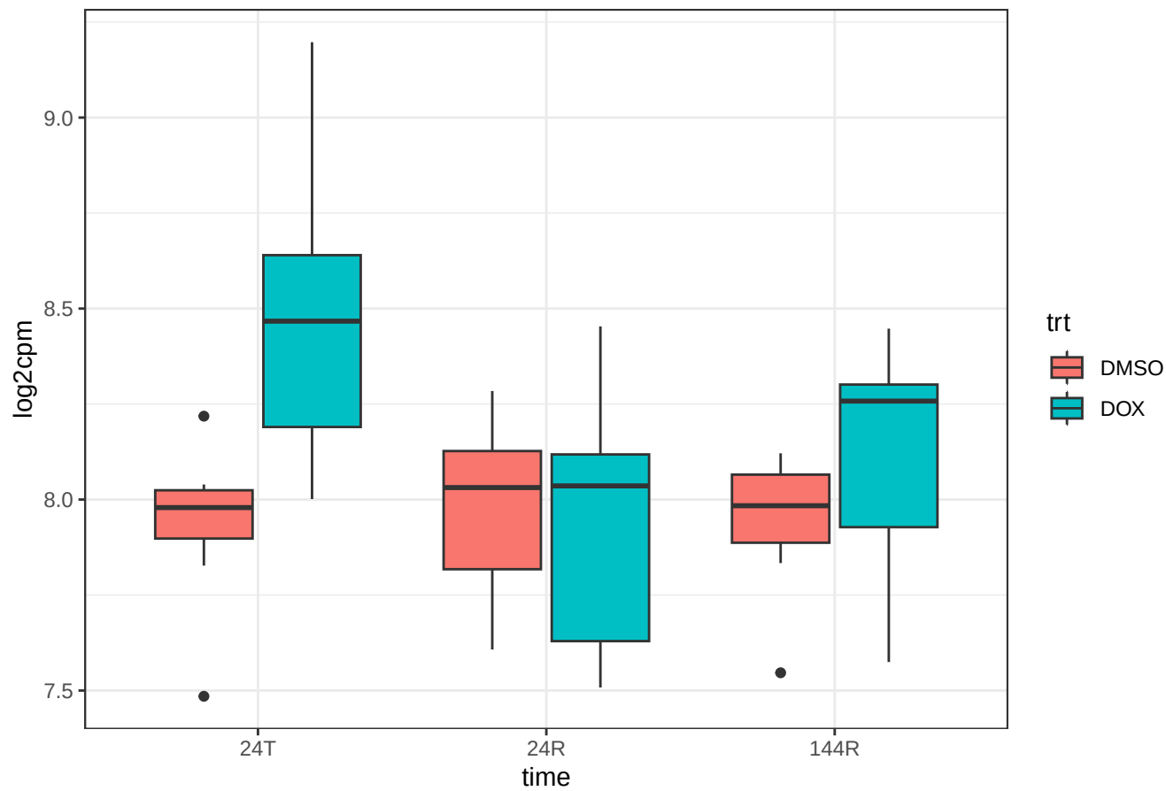
gene 7991 TUSC3 dist 0
