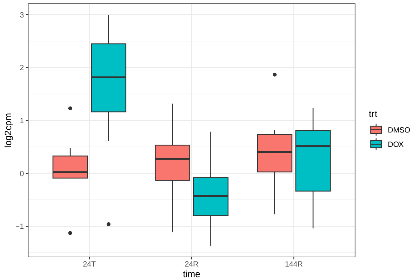
gene 114786 XKR4 dist 0
