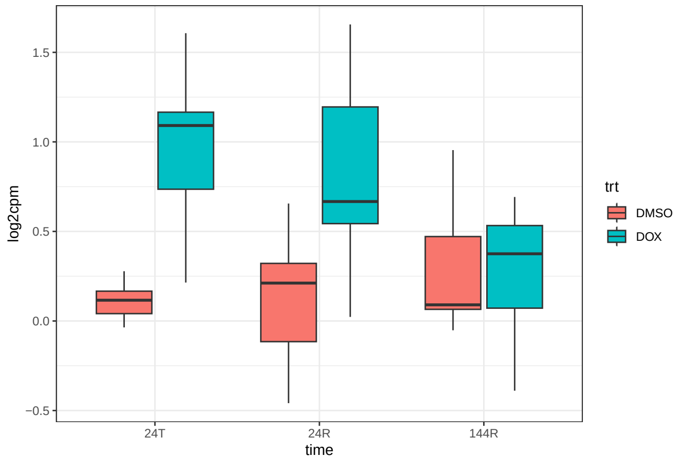
gene 497258 BDNF-AS dist 0
