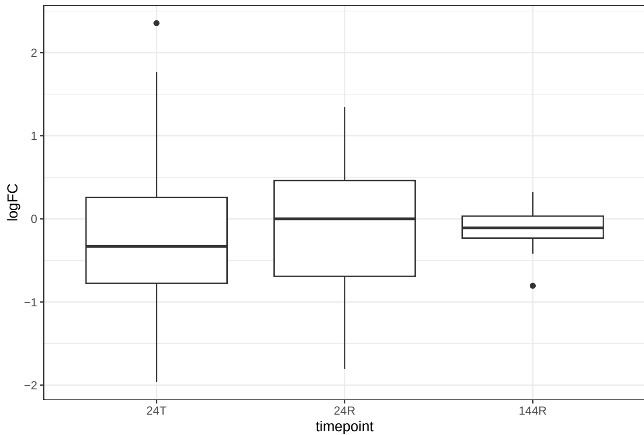
LFC at timepoints of nearest gene to MER61E TE elements in my data
