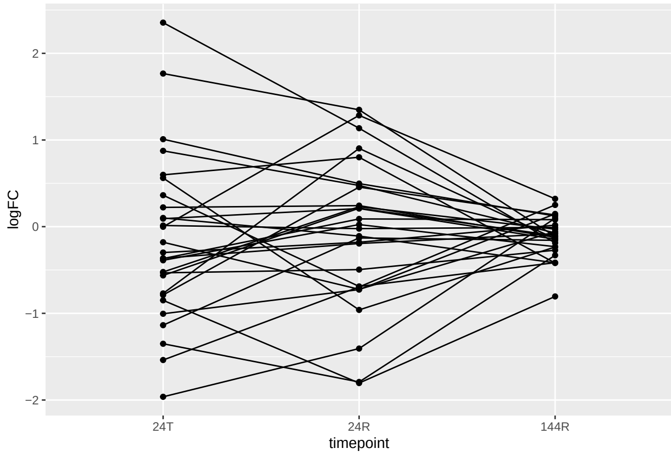
LFC at timepoints of nearest gene to all MER61E TE elements in my data
