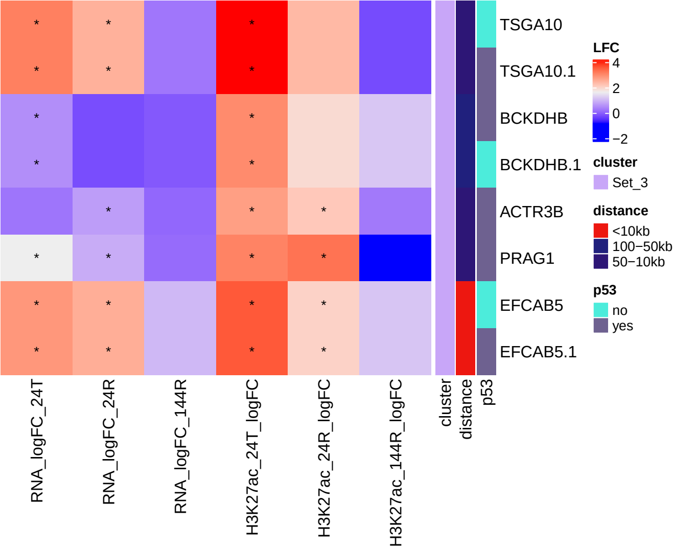
LTR10E H3K27ac assigned gene transition_DOX_only
