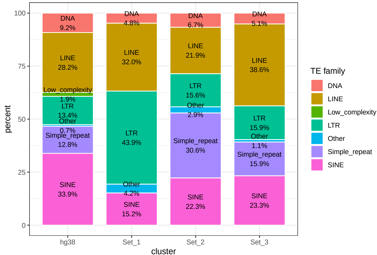
TE Class composition among TE-overlapping ROI summits per set
