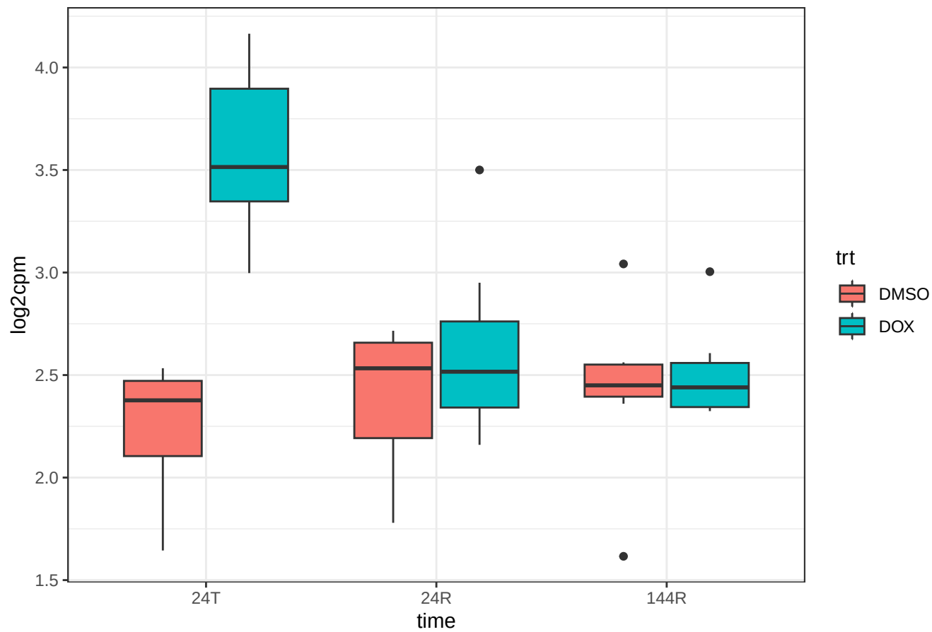
gene 202781 PAXIP1-DT dist 3261
