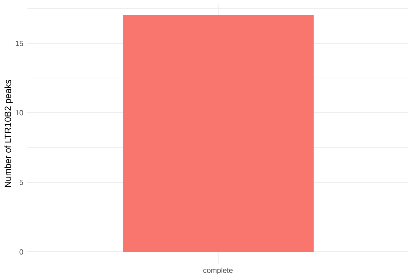
ChromHMM state coverage completeness for LTR10B2
