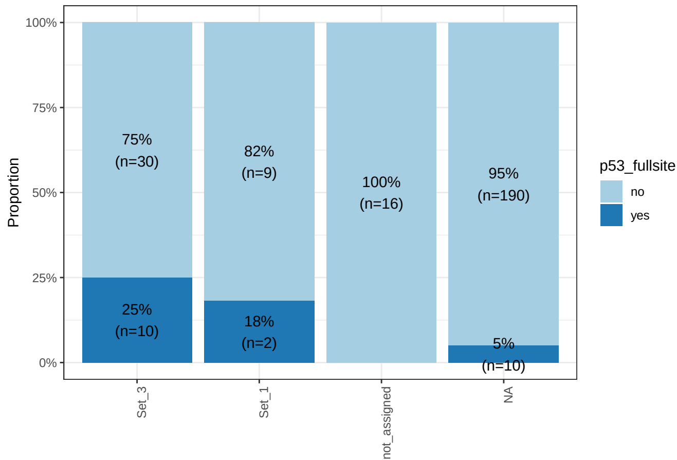
p53 fullsite proportion across MER61E
