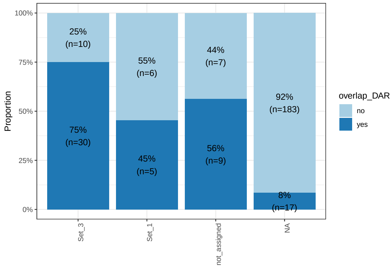
DAR overlap proportion across MER61E
