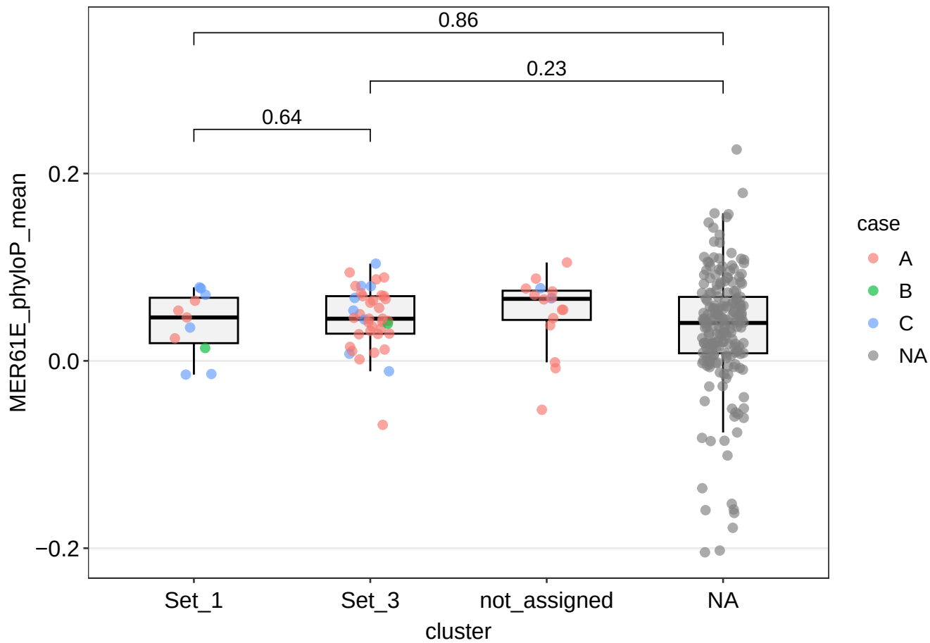
Mean phyloP overlapping MER61E element
